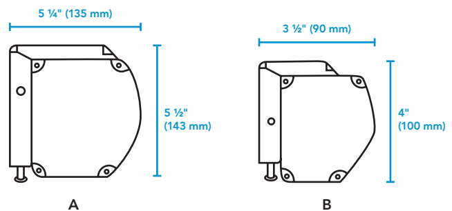
END-CAP VIEW
